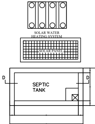
PLAN OF SEPTIC TANK SCALE 1"=2'0"
