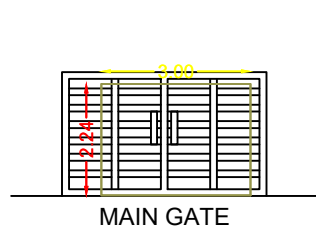
MAIN GATE
