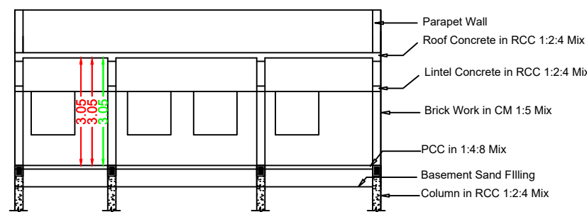
Section RR
