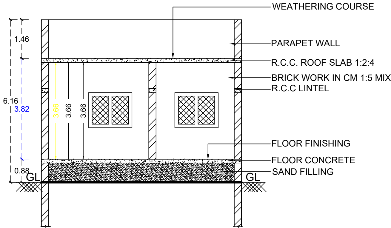
SECTION A1-A1
