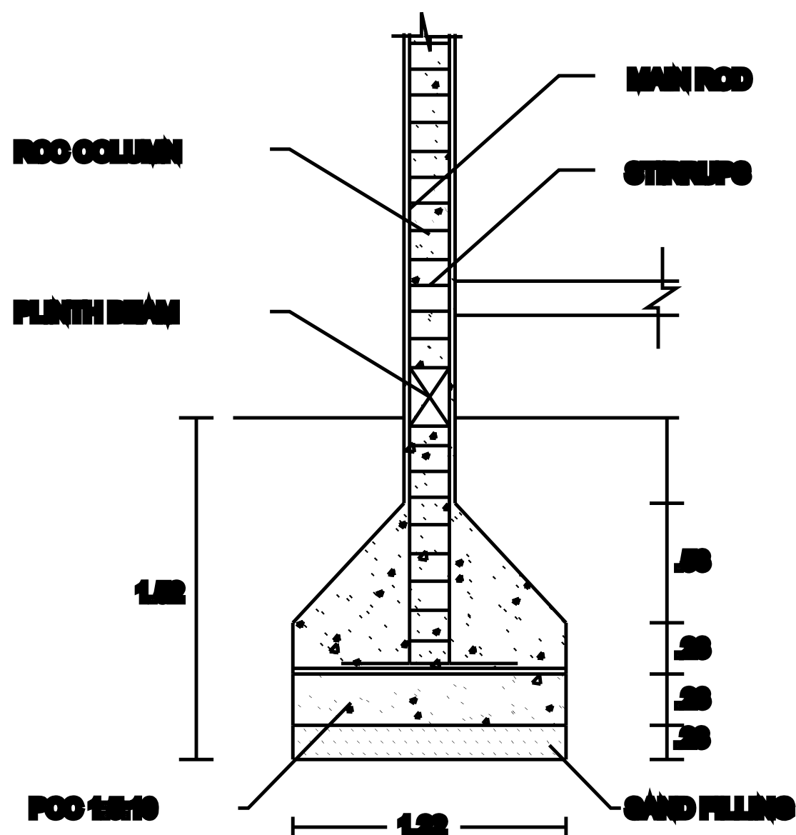
COLUMN DETAILS
