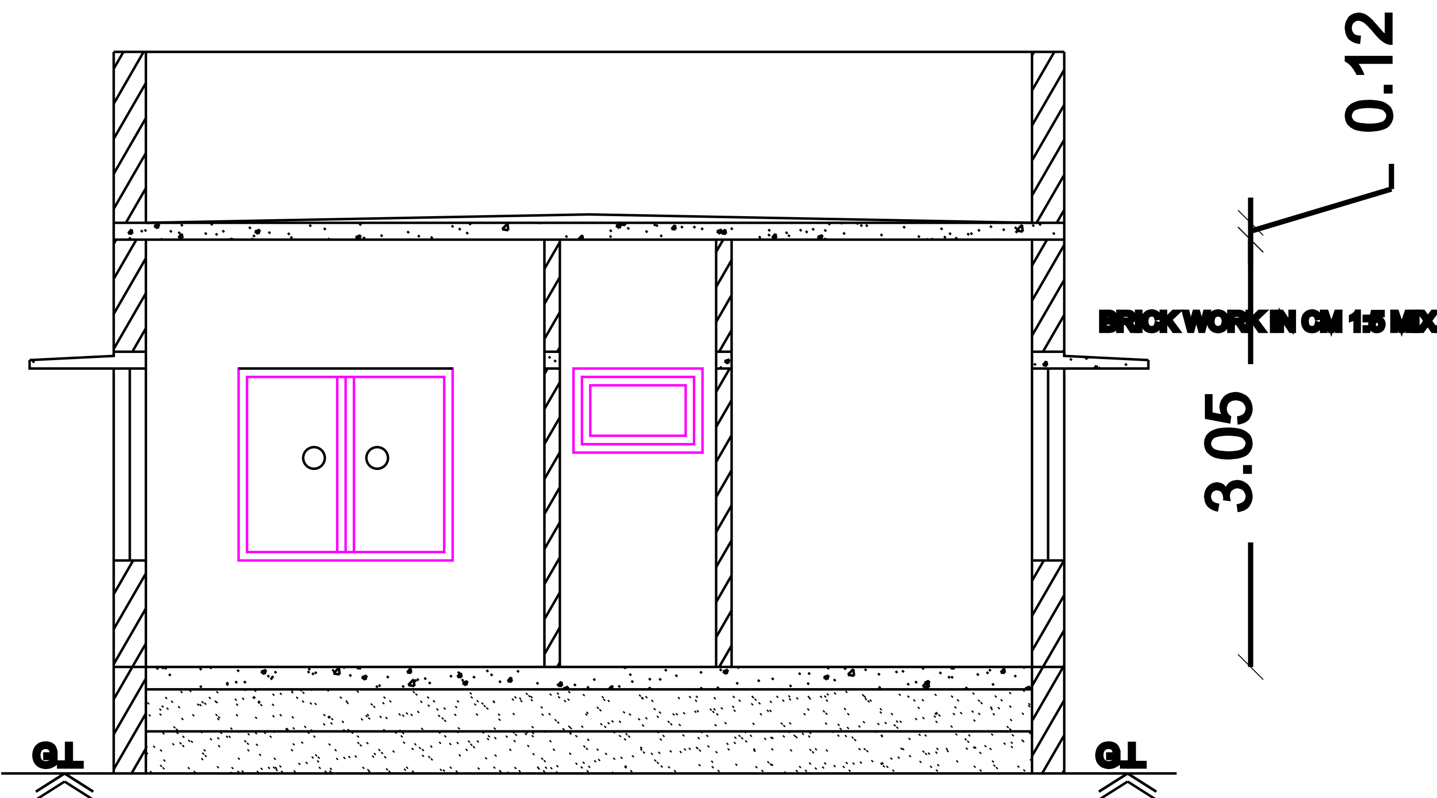
Section on-"AA"
