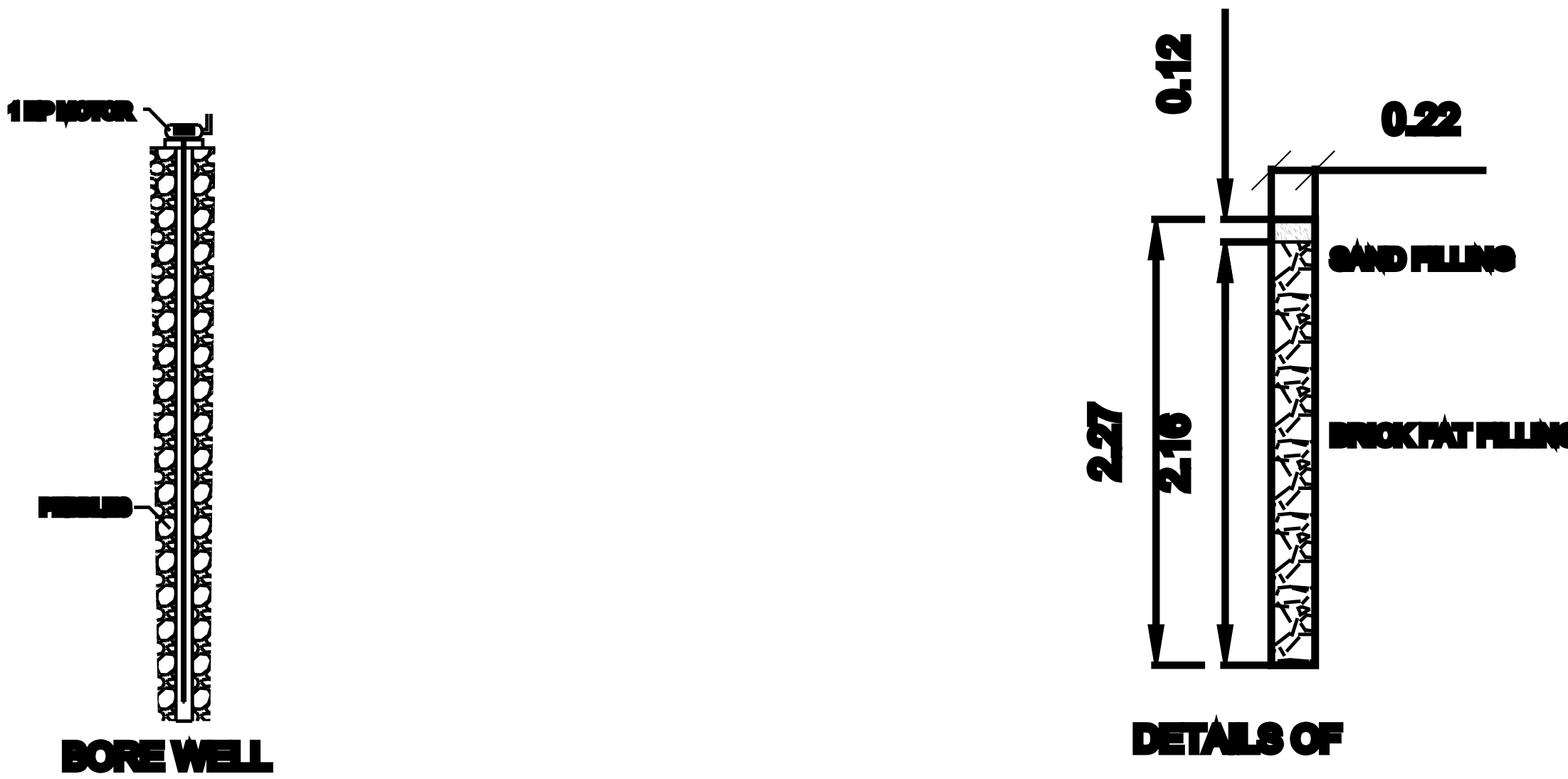
Section on-"AA"
