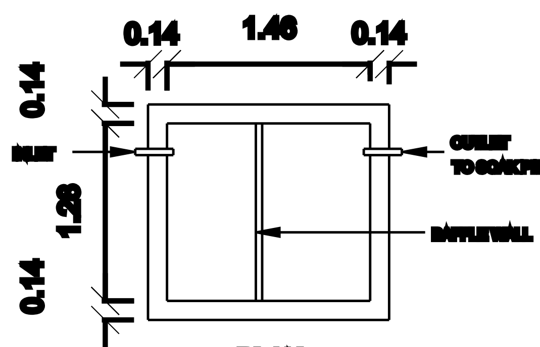
PLAN SEPTIC TANK
