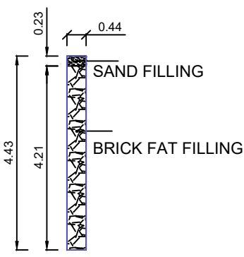
DETAILS OF PERCULATION PIT
