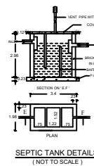
SEPTIC TANK DETAILS (NOT TO SCALE)
