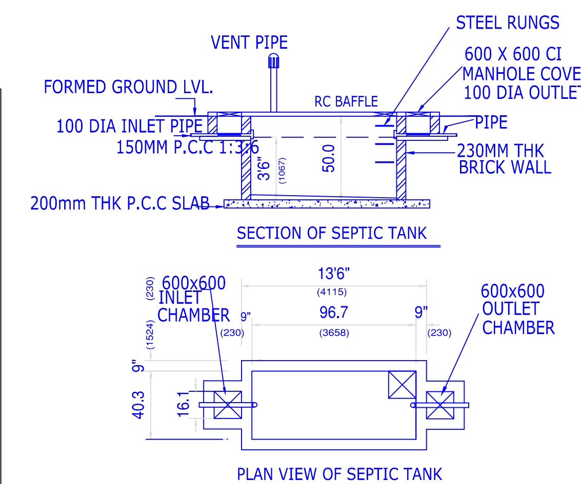
PLAN VIEW OF SEPTIC TANK
