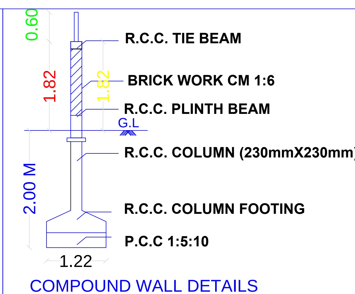
COMPOUND WALL DETAILS
