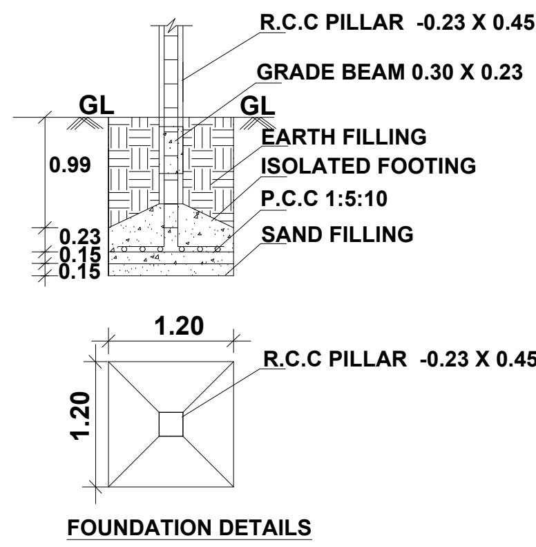
FOUNDATION DETAILS
