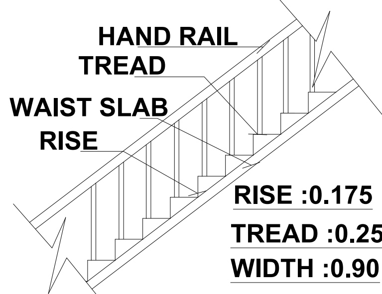
STAIRCASE DETAILS
