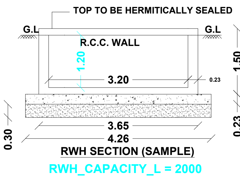
RWHS SECTION (SAMPLE)
