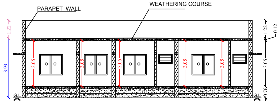
Section on-"AA"
