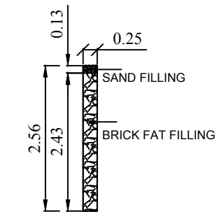
DETAILS OF PERCULATION PIT
