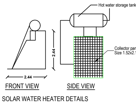
SOLAR WATER HEATER DETAILS
