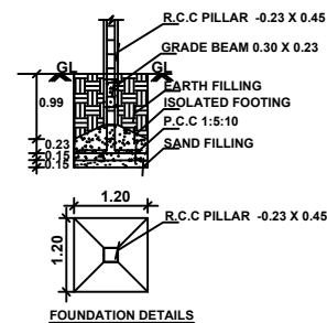
FOUNDATION DETAILS
