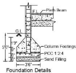
Foundation Details
