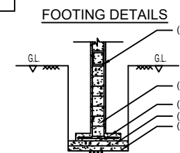
FOOTING DETAILS SECTION
