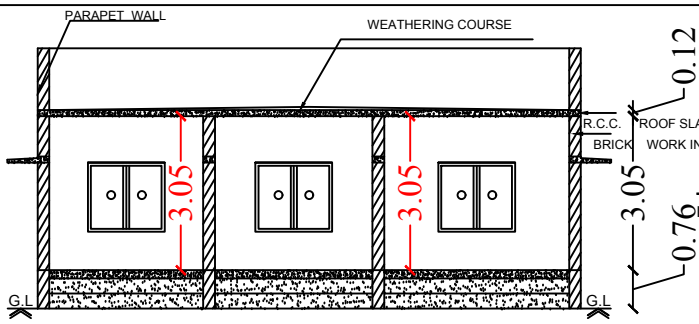
Section on-"AA"
