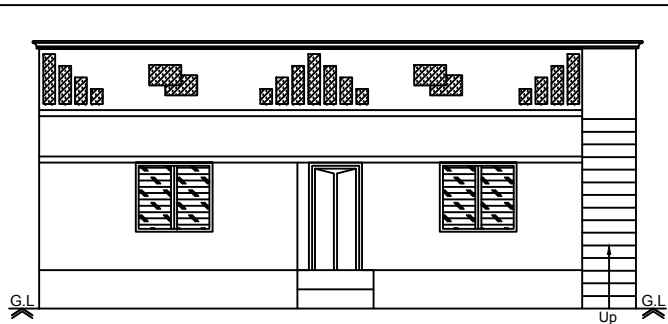
Front Elevation
