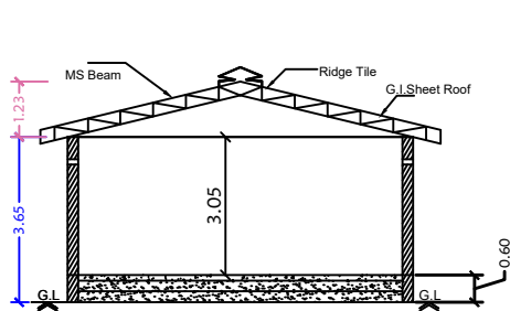
Section on-"AA"
