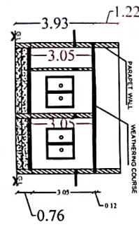
Section on "AA"
