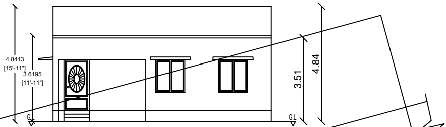
ELEVATION ON EAST SIDE
