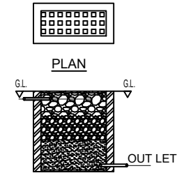
RAINWATER STORAGE PIT DETAILS
