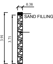
DETAILS OF PERCULATION PIT
