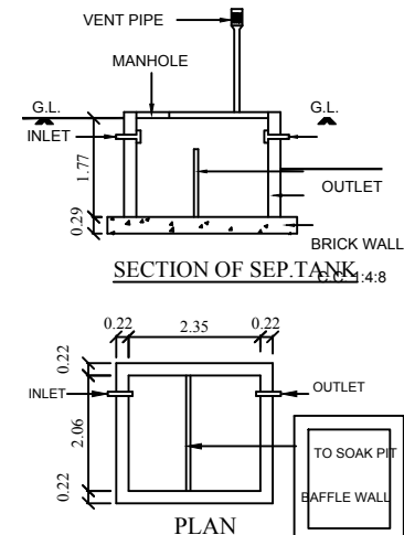
SECTION OF SEP. TANK
