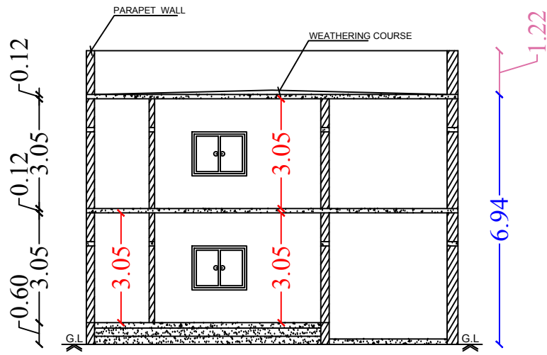
Section on-"AA"
