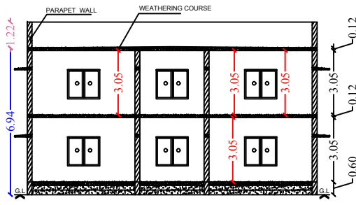
Section on-"AA"
