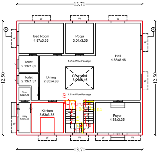
Existing - Ground Floor
