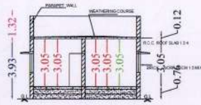
Section on-AA'
