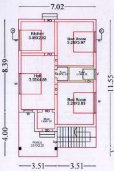
Floor - Ground
