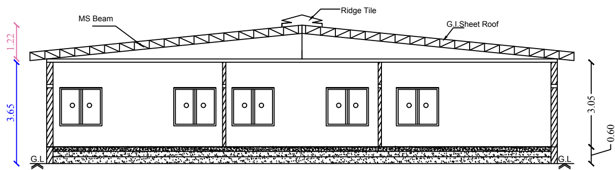
Section on-"AA"
