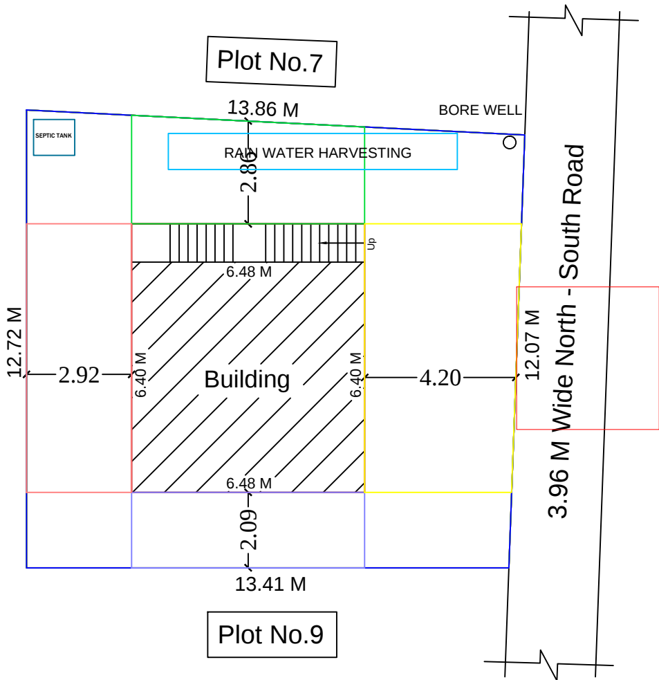
SITE PLAN
