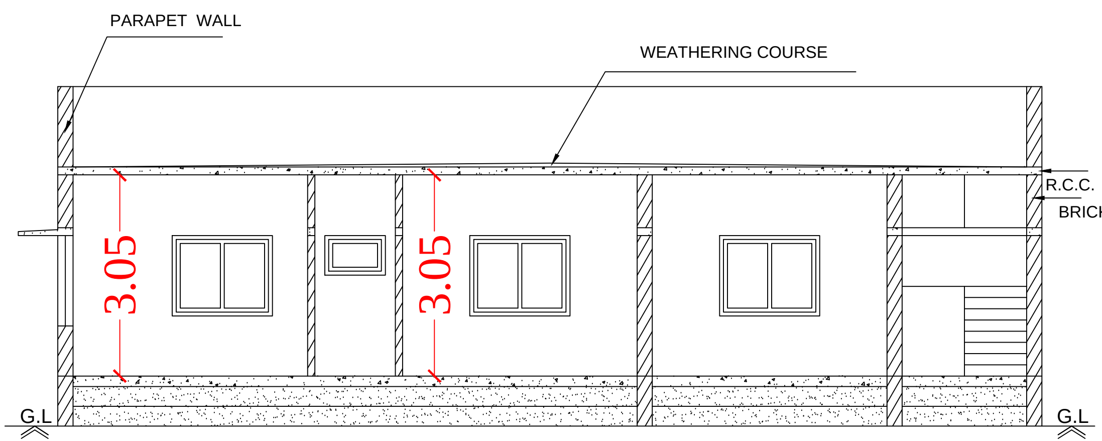
Section on-"AA"
