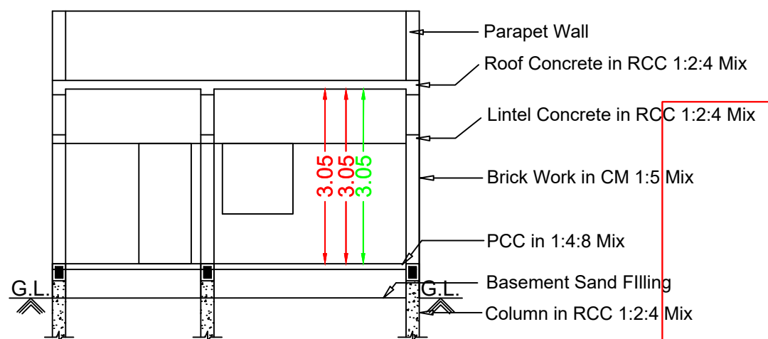
Section RR
