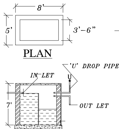
SEPTICTANK DETAILS
