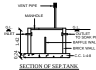
SECTION OF SEPTIC TANK
