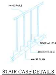
STAIR CASE DETAILS
