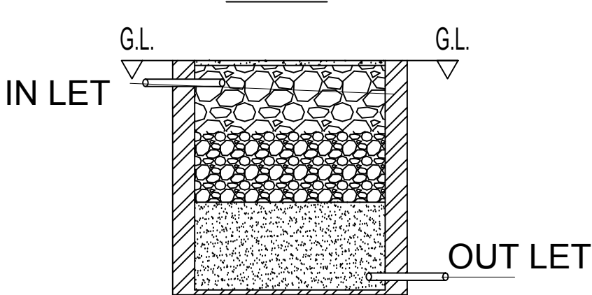
RAINWATER STORAGE PIT DETAILS
