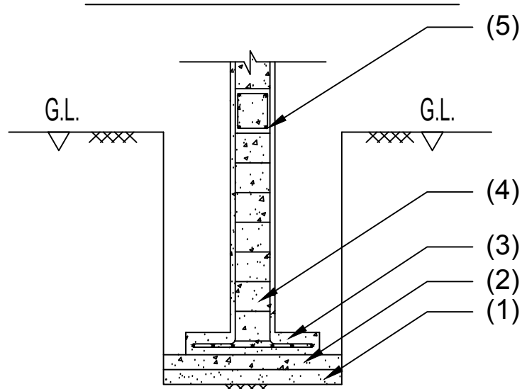
FOOTING DETAILS
