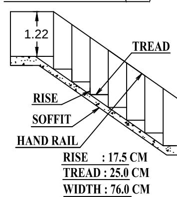
STAIRCASE DETAILS (NTS)
