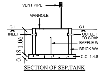
SECTION OF SEP. TANK
