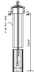
BOREWELL DETAILS
