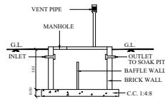
SECTION OF SEPT.TANK
