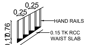
DETAILS OF STAIR CASE
