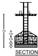
SECTION (BLOCK-1)
