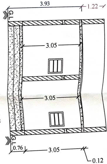
Section on-"AA"
