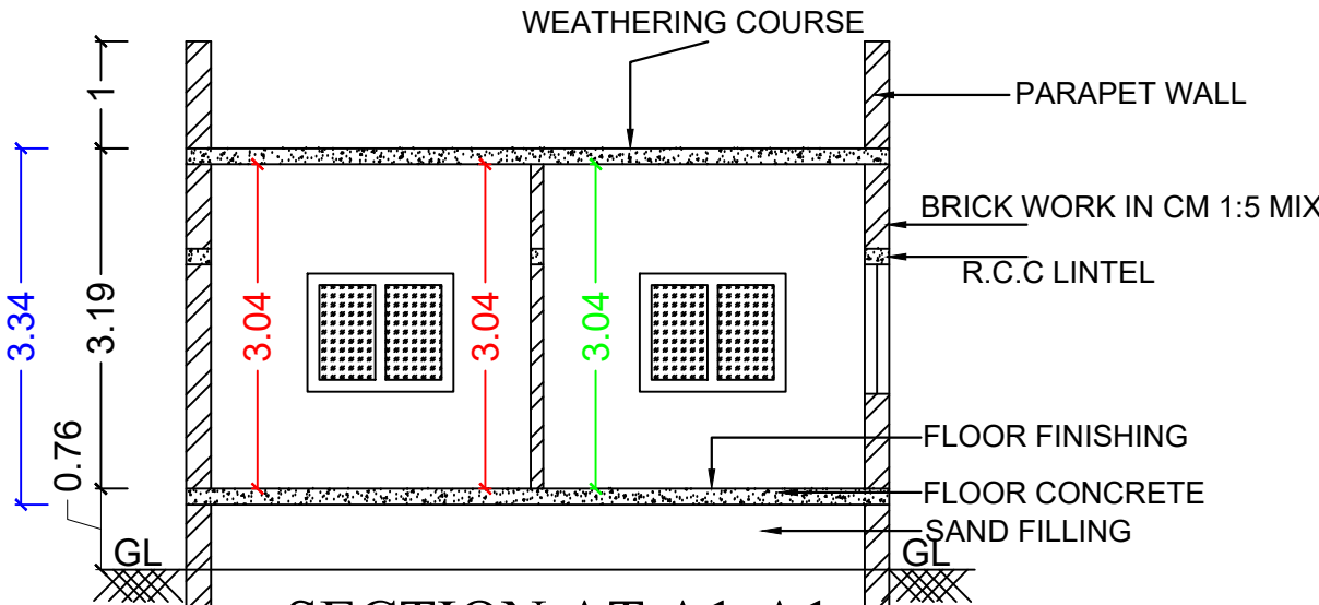
SECTION AT A1-A1
