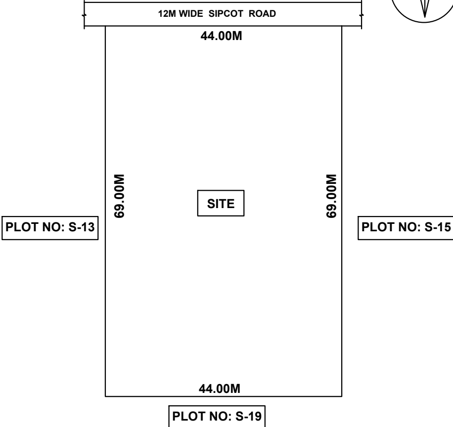
TOPO SKETCH
