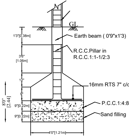
FOUNDATION DETAILS
