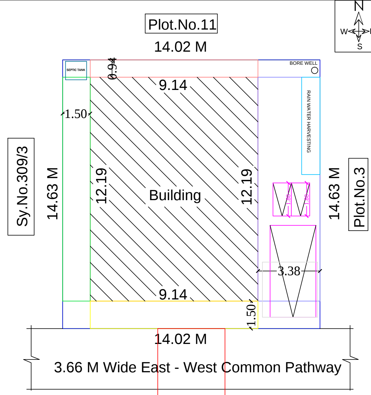
SITE PLAN
