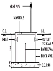
SECTION OF SEP.TANK
