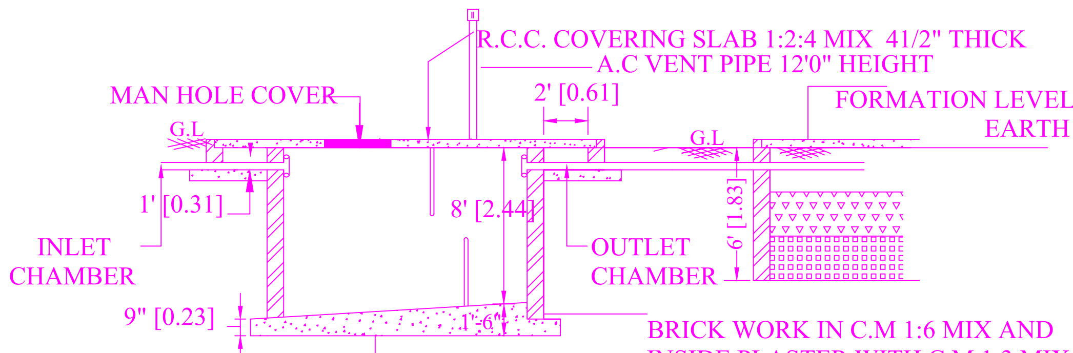
SEPTIC TANK
