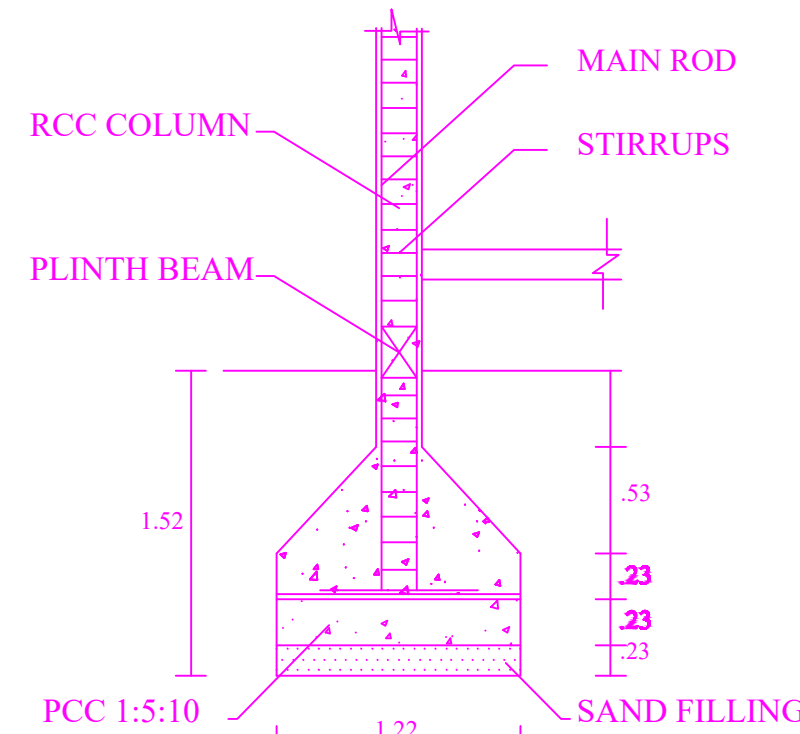
COLUMN DETAILS
