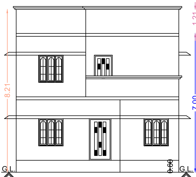
Front Elevation
