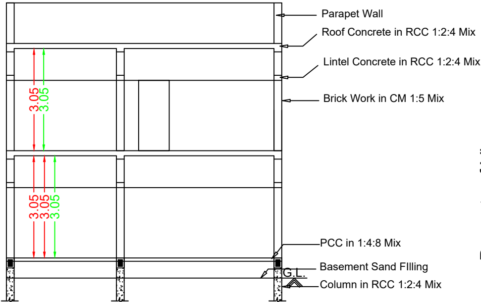
Section RR
