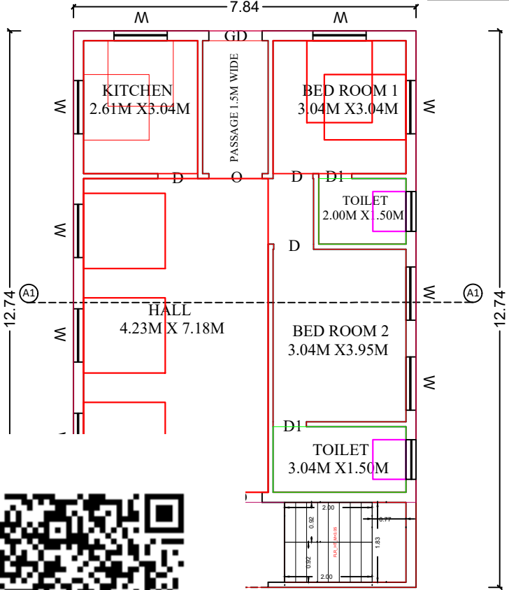
FLOOR PLAN
