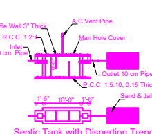
Septic Tank with Dispersion Trench
