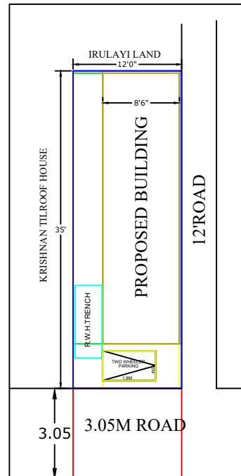
SITE PLAN
