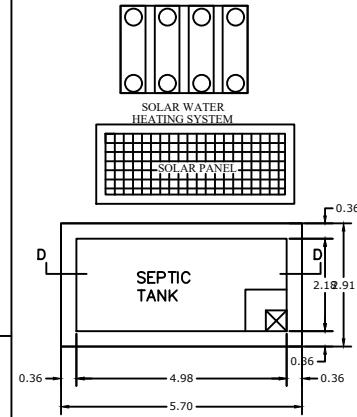
PLAN OF SEPTIC TANK SCALE 1"=2'-0"
