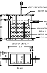
SEPTIC TANK DETAILS (NOT TO SCALE)
