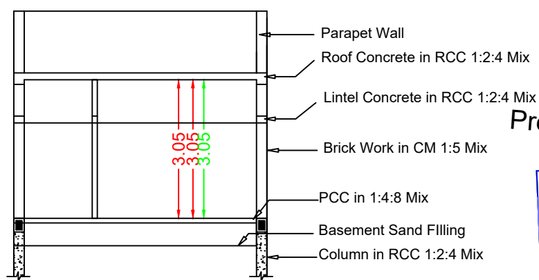
Section RR
