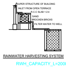
Section RR
