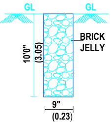
PERCOLATION PIT
