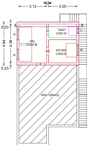
RAIN WATER HARVESTING SYSTEM RWH_CAPACITY_L=1000LTRS
