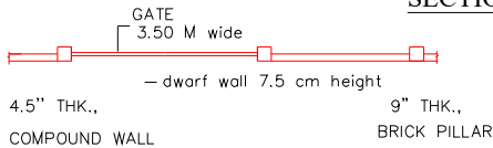
COMPOUND WALL PLAN
