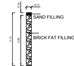
DETAILS OF PERCUSSION PIT
