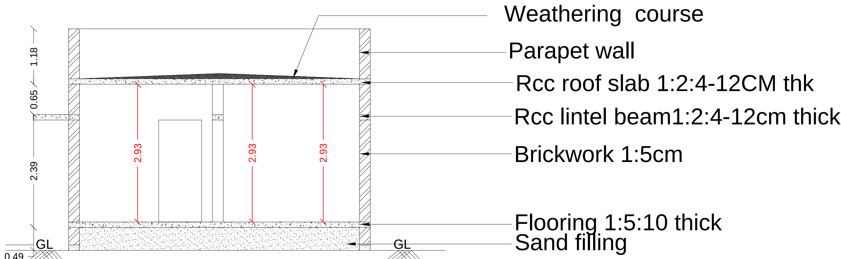
SECTION-AA
