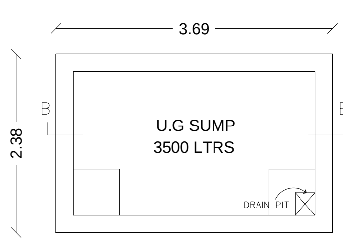
PLAN OF SUMP
