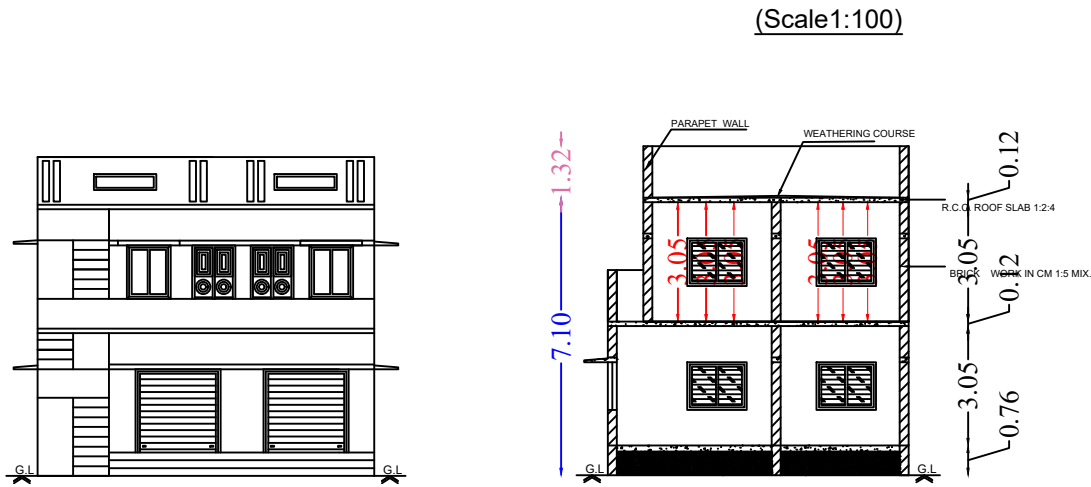
Front Elevation
