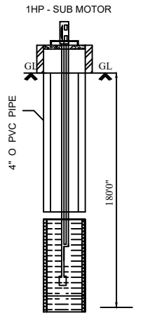
Bore Well Details
