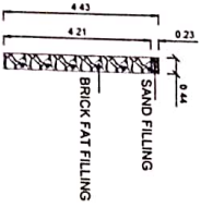
DETAILS OF PERFORATION PIT
