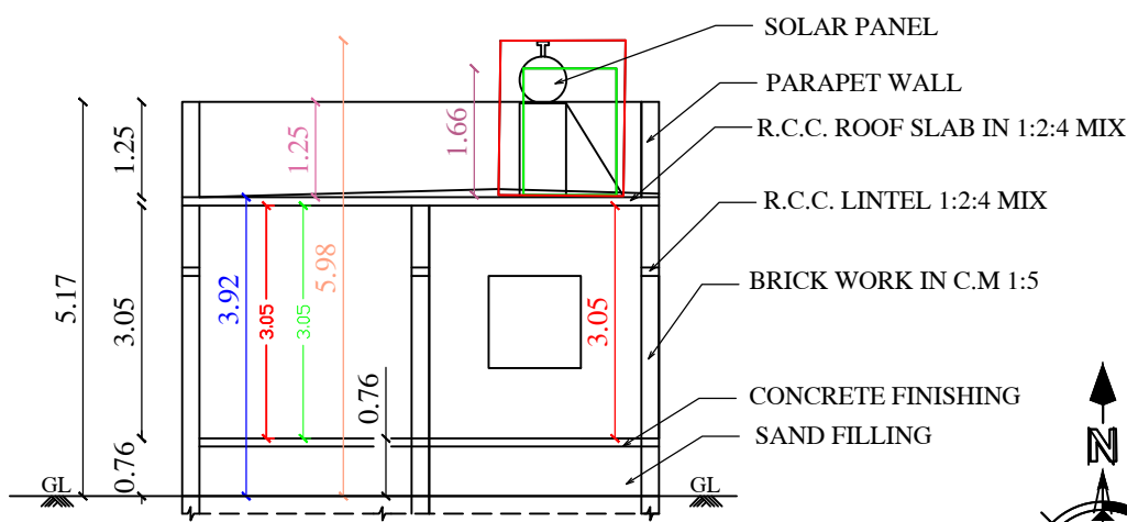
CUT SECTION ON "AA"
