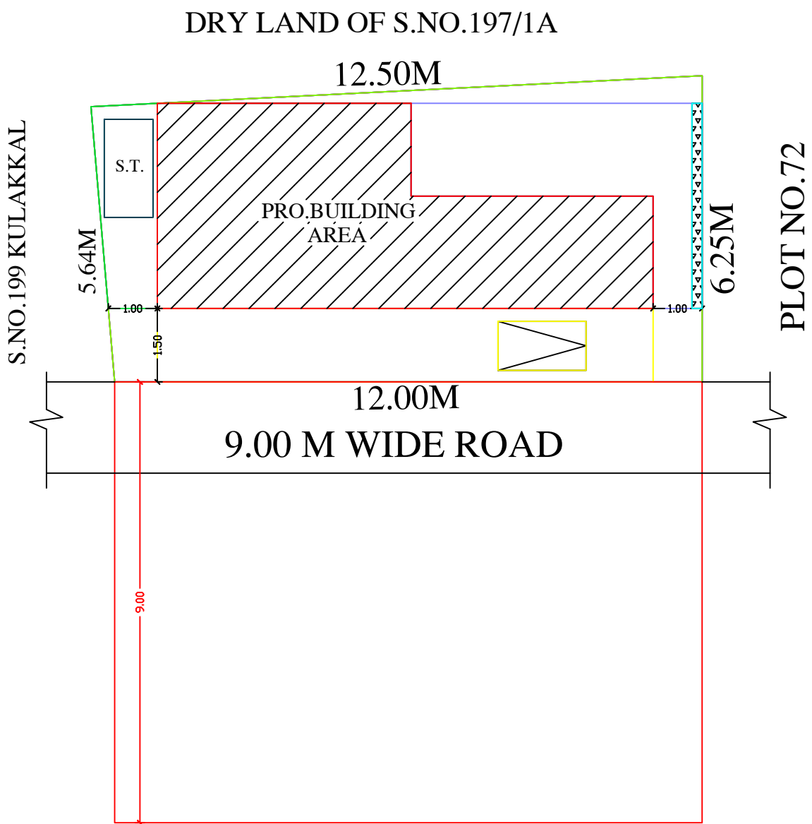
SITE PLAN
