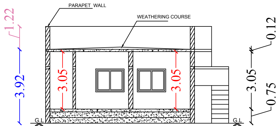
Section on-"AA"
