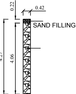
DETAILS OF PERCULATION PIT
